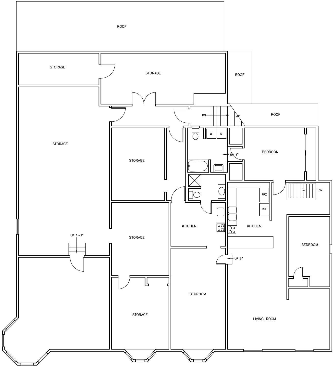
A SECOND FLOOR PLAN SCALE: 1/4" = 1'-0" D:\CAD\0803
