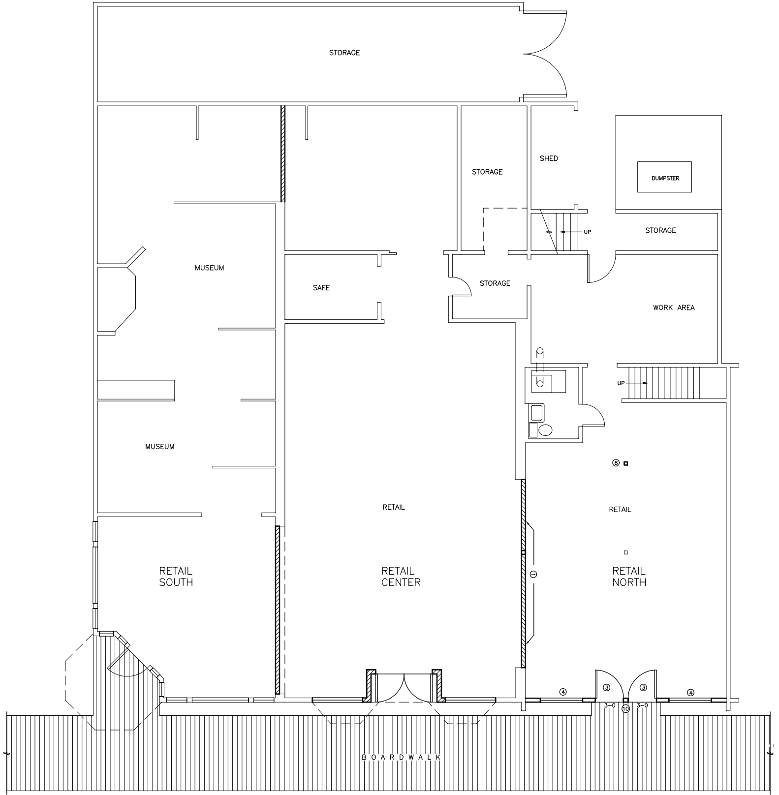
A NEW 1ST FLOOR PLAN SCALE: 1/4" = 1'-0" D:\CAD\0803
